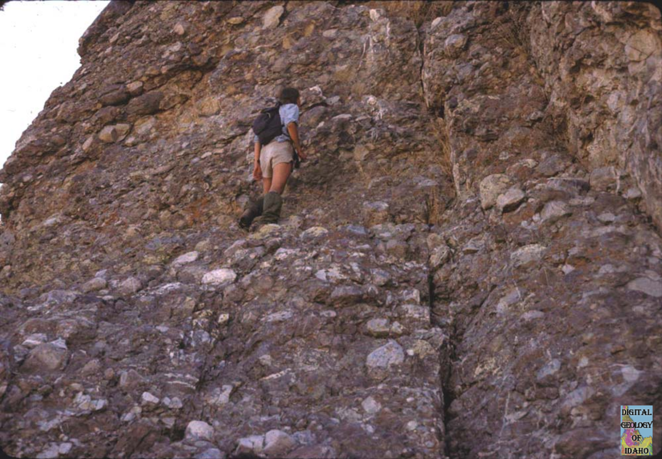
Cobble conglomerate in Scout Mountain Member Pocatello Formation, south of Portneuf Gap.
