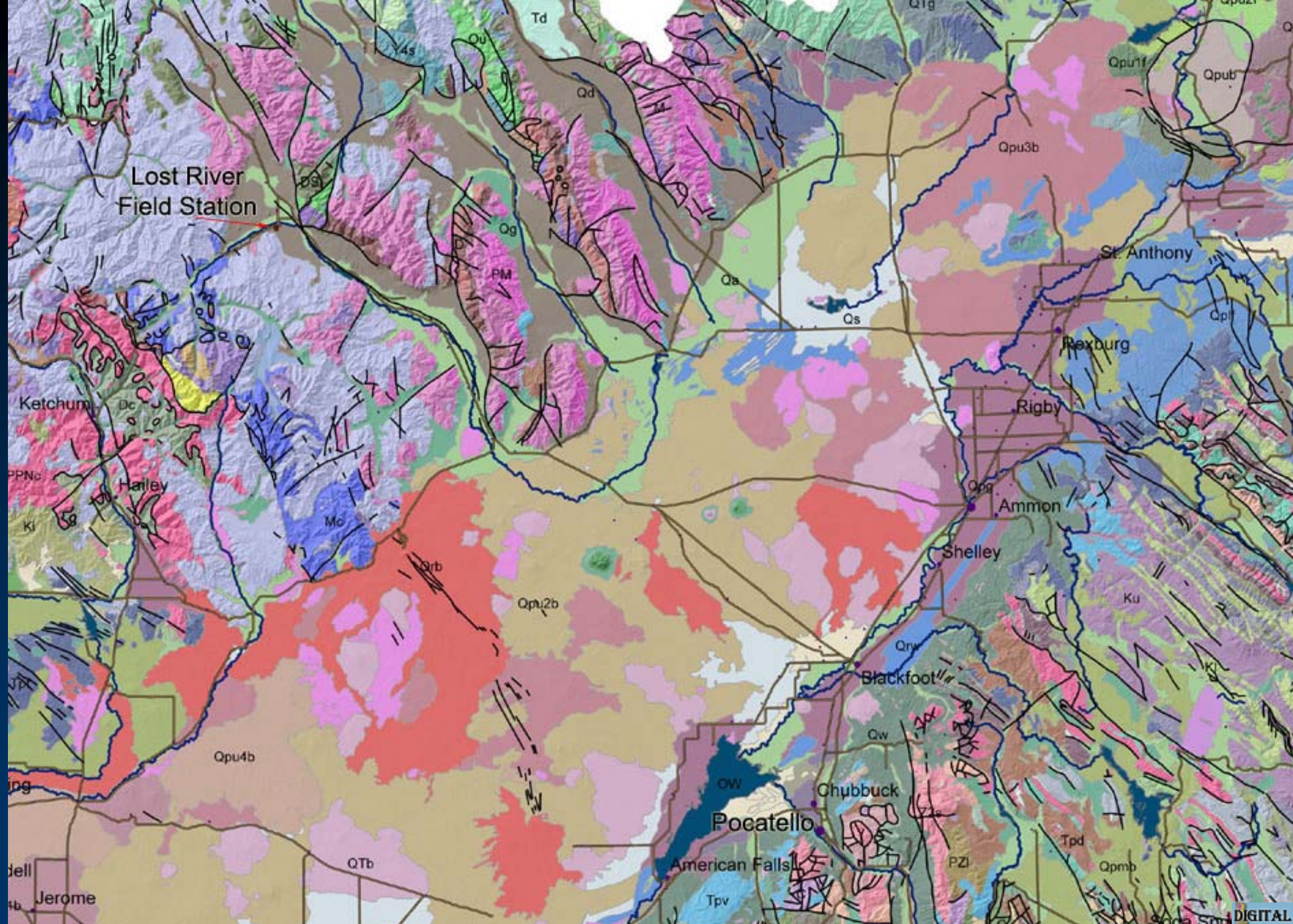
Geologic Map of the same area as first slide.
