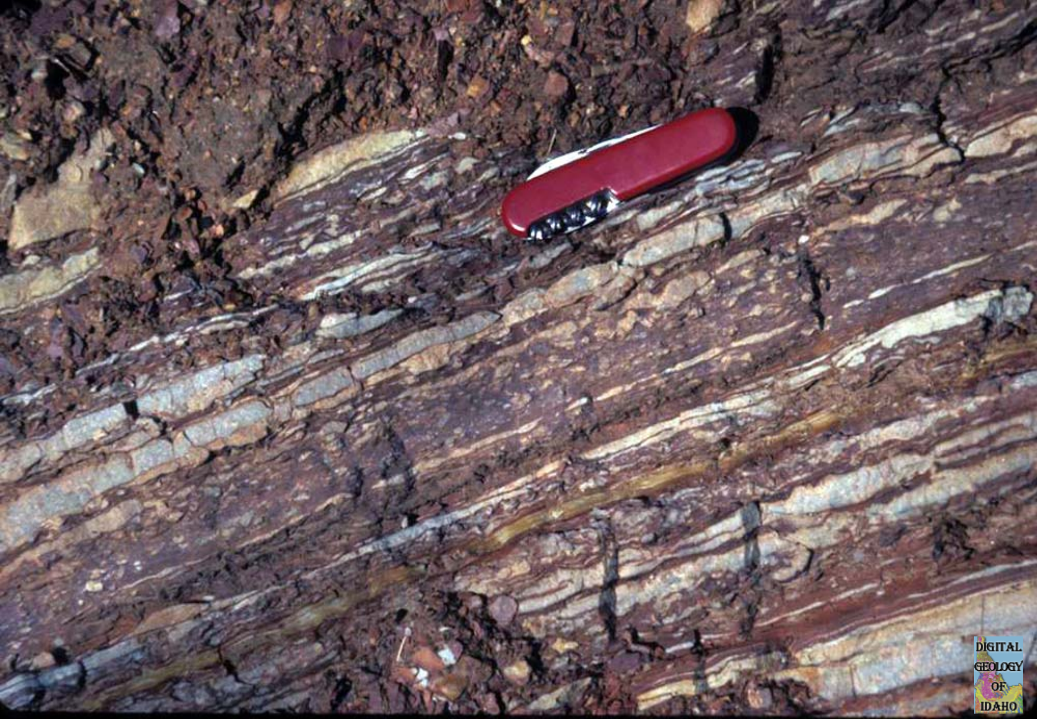
Papoose Creek Formation, Brigham Group, north of Huntsville, Utah
